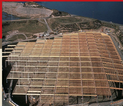
Red-H™ trusses—60 feet long and up to 6 feet deep—form the structural backbone of this 12-acre reservoir cover, which was specially engineered to withstand both vertical and horizontal loads.
