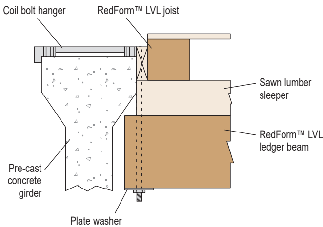
Detail B2
