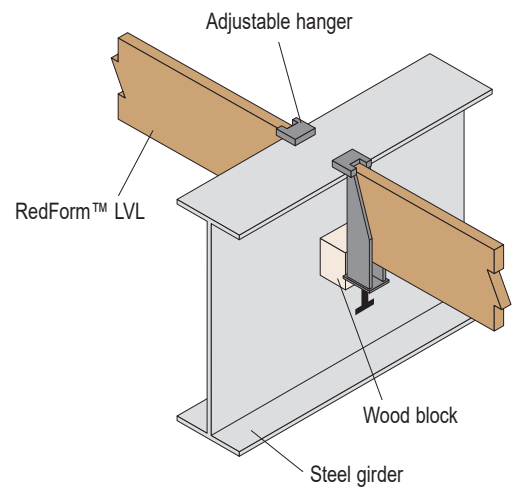
Detail C1
